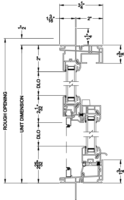
3500 SINGLE HUNG WINDOW (9107) Vertical Section
