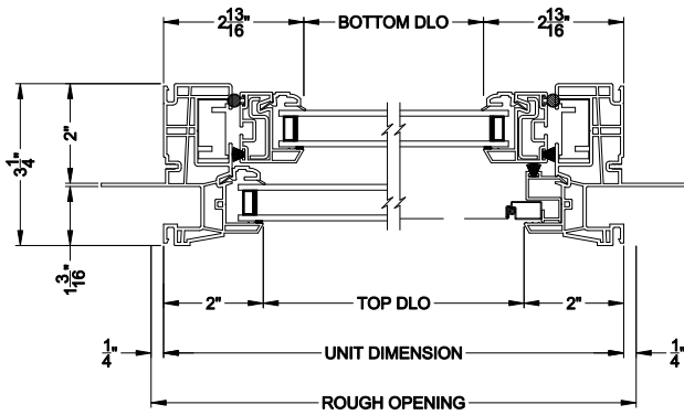
3500 SINGLE HUNG WINDOW (9109) Horizontal Section - DP50 upgrade
