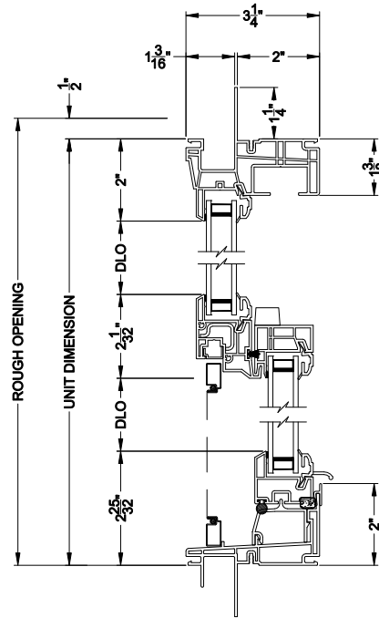
3500 SINGLE HUNG WINDOW (9109) Vertical Section - DP50 upgrade
