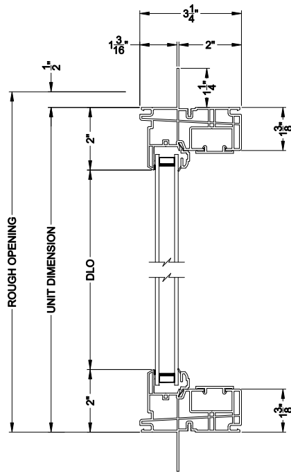
3500 SH PIC / TRANS WINDOW (9310) Vertical Section
