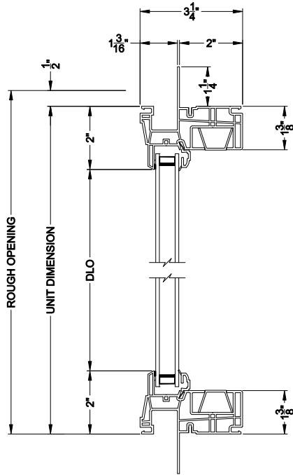
3500 PICTURE / TRANSM WINDOW (9311) Vertical Section - J-Channel
