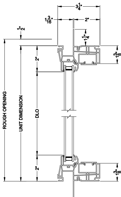
3500 PICTURE / TRANSM WINDOW (9311) Vertical Section
