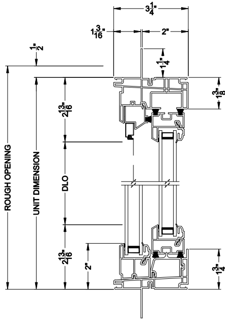
3500 SLIDER WINDOW (9407) Vertical Section - Non J-Channel
