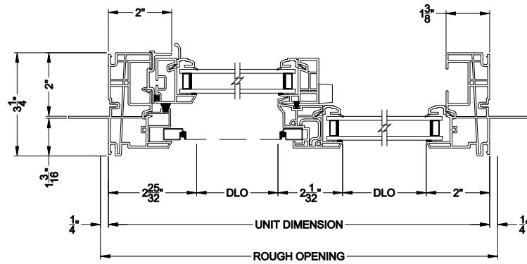
2500 SINGLE SLIDER WINDOW (9407) Horizontal Section
