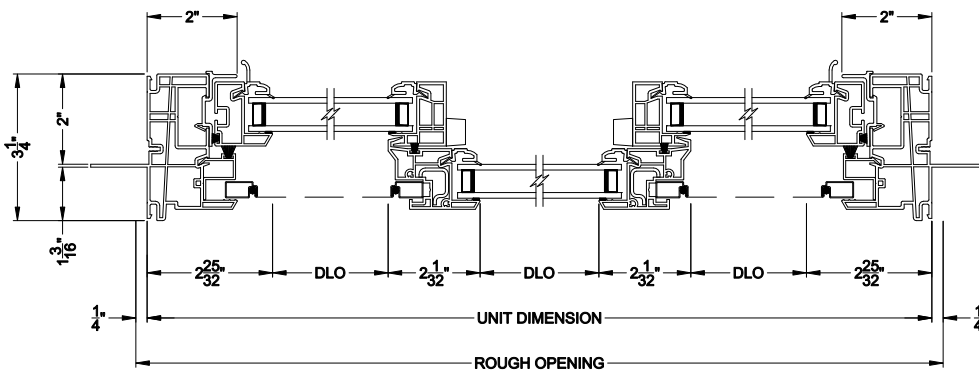
2500 TRIPLE SLIDER WINDOW (9407) Horizontal Section
