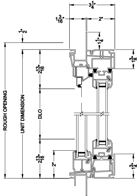
3500 SLIDER WINDOW (9408) Vertical Section
