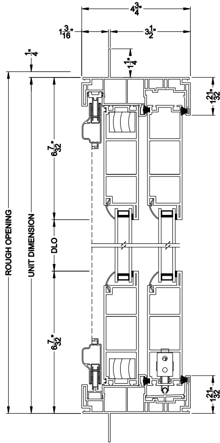
3500 FRENCH SLIDING PATIO DOOR 2 PANEL (9702) Vertical Section
