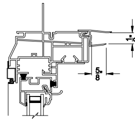
1/2" DRYWALL RECEPTOR Head Section Detail
