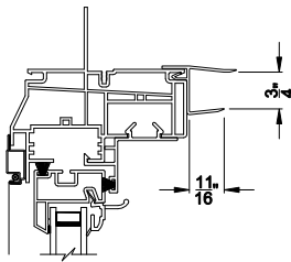
3/4" TRIM RECEPTOR Head Section Detail
