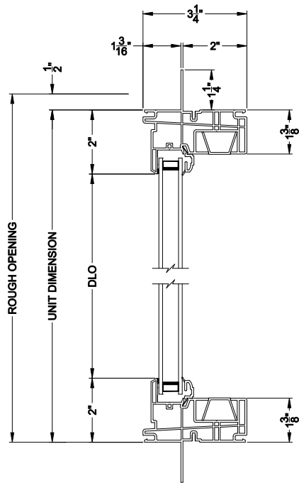
3500 SH PIC / TRANS WINDOW (9310) Vertical Section - Non J-Channel
